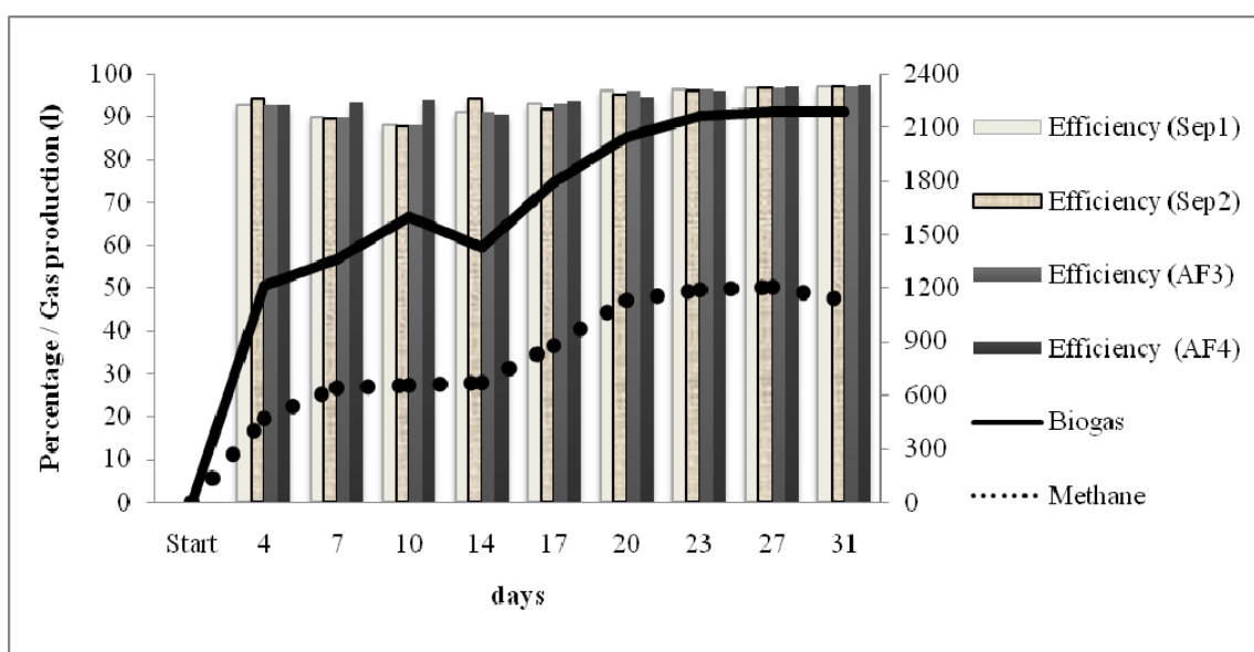
Figure 3. The comparison of biogas and methane production during the experiment.
