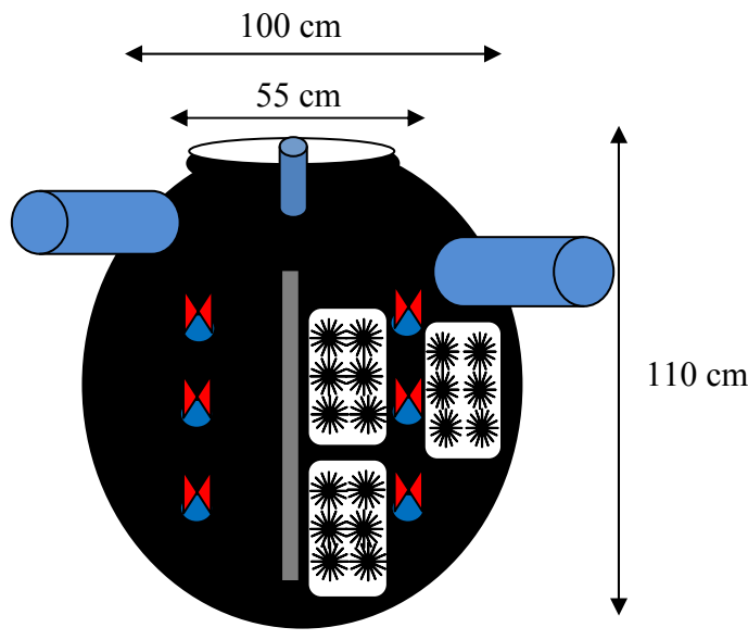
Figure 2. Schematic of pilot scale anaerobic digester
