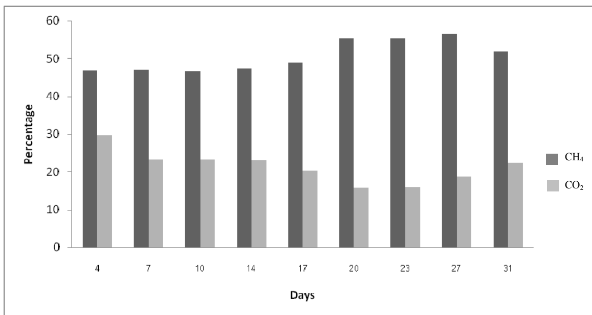
Figure 4. The relation of CH 4 and CO 2 from anaerobic digestion
