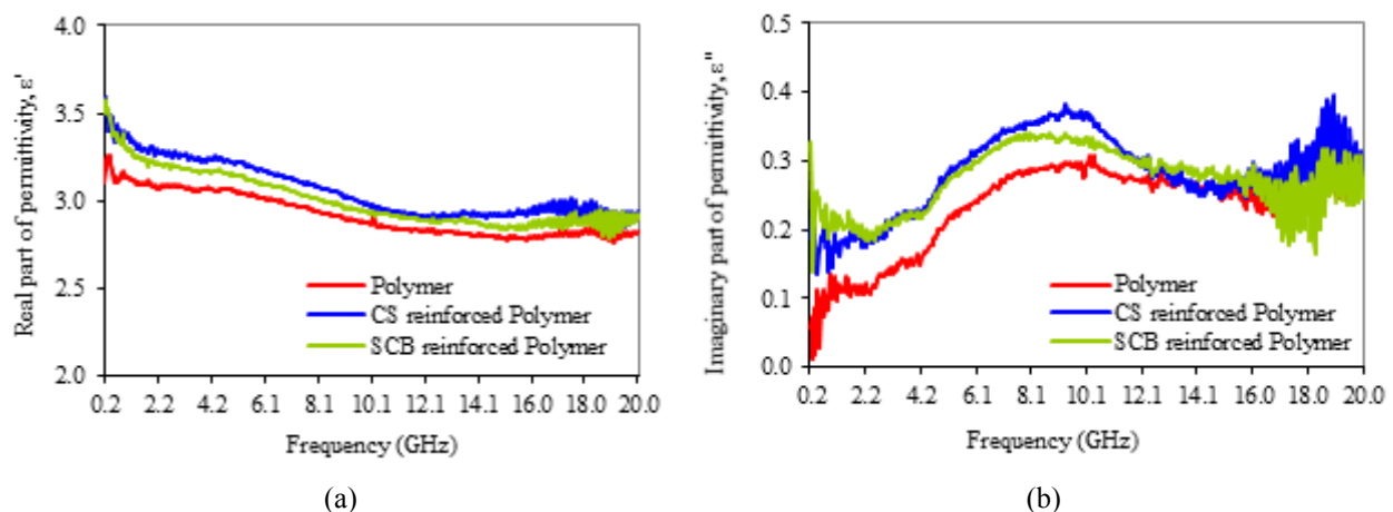
Figure 6. Complex permittivity in the function of frequency range 200 MHz-20 GHz (a) Frequency dependent of real part, \epsilon' , of complex permittivity and (b) Frequency dependent of imaginary part, \epsilon'' , of complex permittivity
