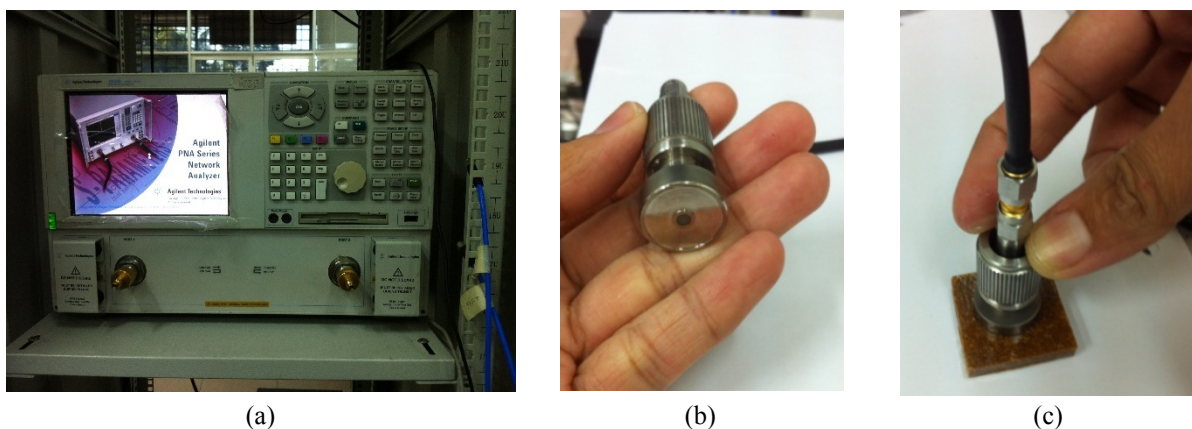
Figure 4. (a) Agilent E8362B PNA series network analyser, (b) High temperature dielectric probe and (c) Dielectric properties measurement
