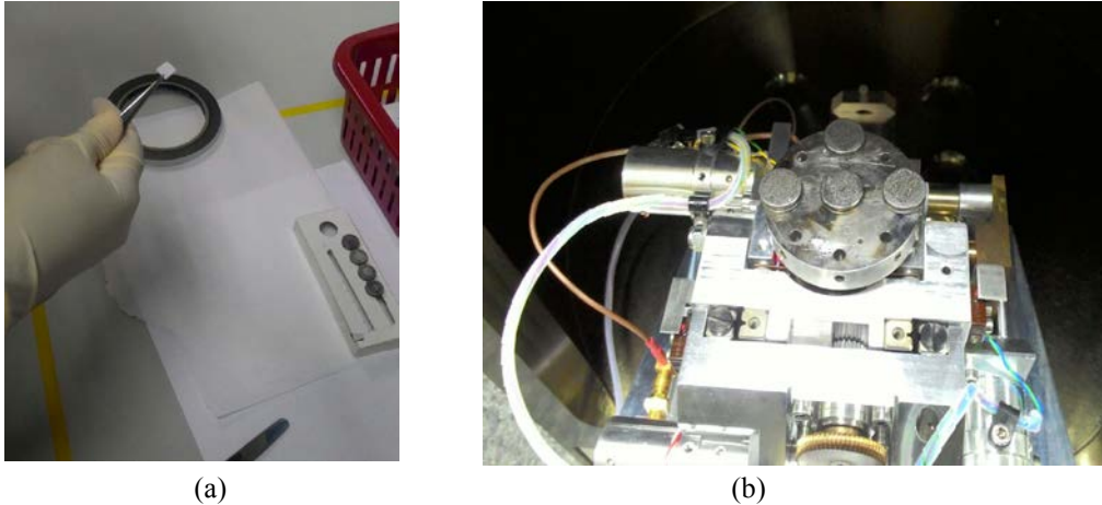
Figure 3. (a) Powder specimens preparation using double coated carbon conductive adhesive tape and cylindrical stubs and (b) Placement of coated powder specimens in the scanning electron microscope
